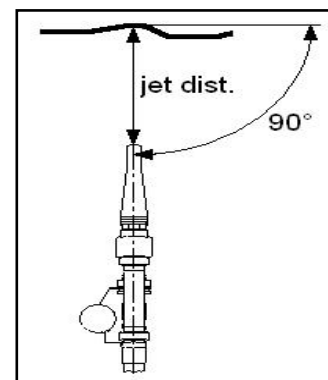
Figure 4 Stand-off distance and nozzle angle
